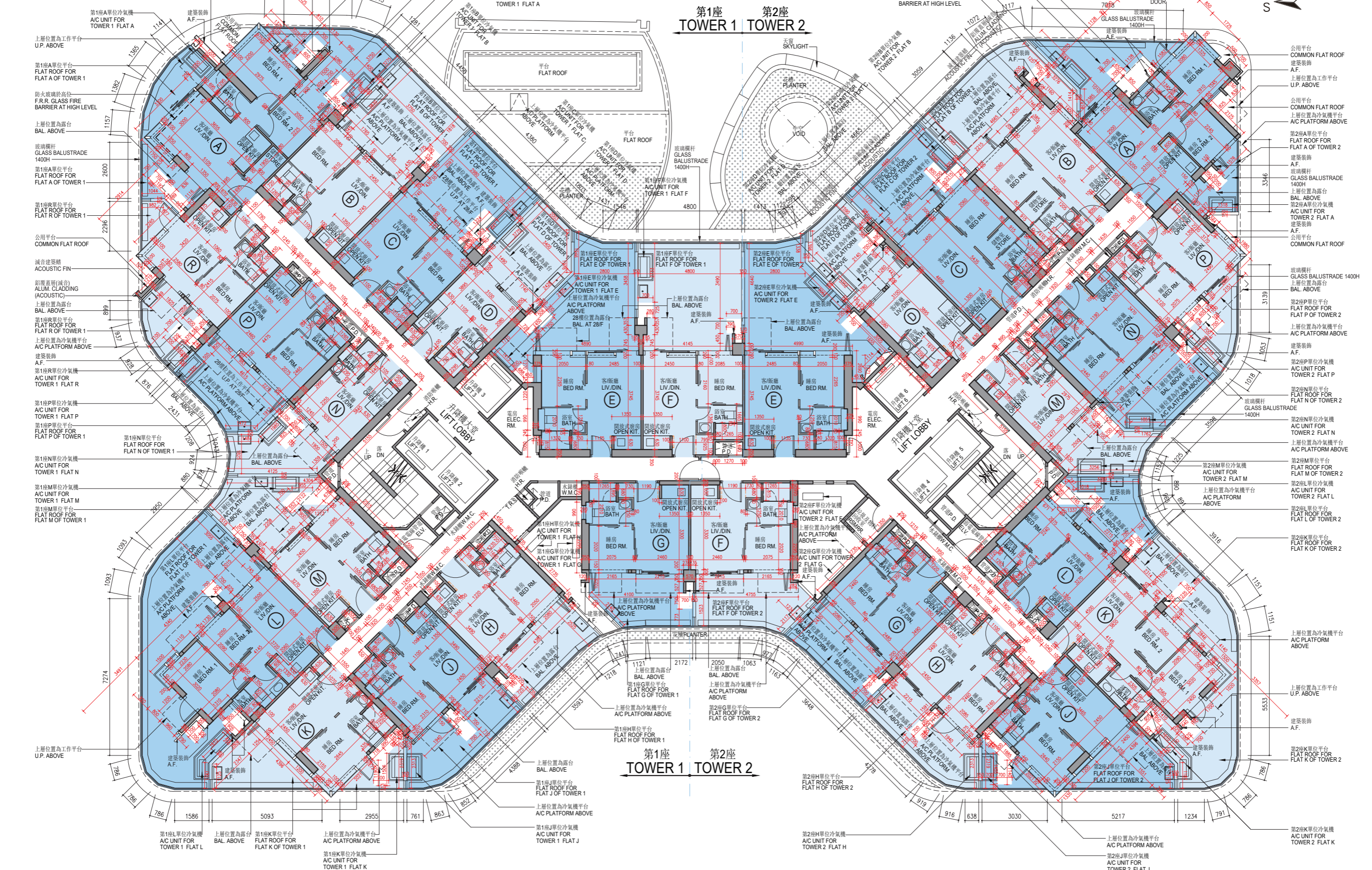
3樓平面圖 3/F FLOOR PLAN
