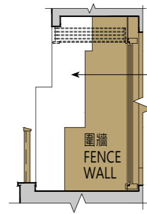
圍牆立面圖 A Elevation A of Fence Wall
