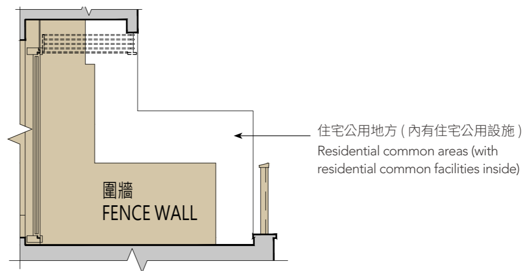
圍牆立面圖 A Elevation A of Fence Wall
